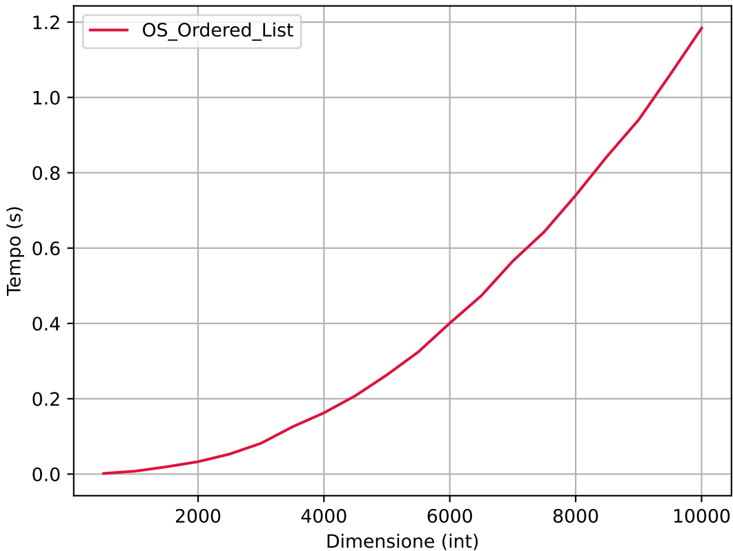
OS Ordered List - Test Casual Rank
